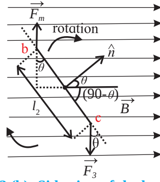
Fig. 10.12 (b): Side view of the loop abcd at an angle \theta .
