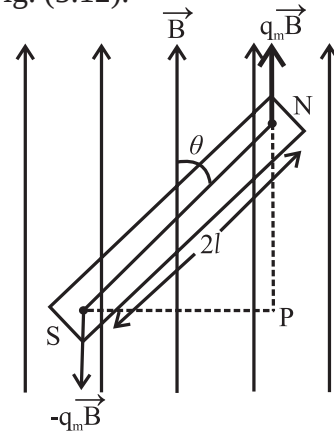
Fig. 5.12: Magnet vibrating in a uniform magnetic field.
