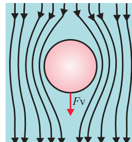
Fig 2.31: Spherical object moving through a viscous medium.
