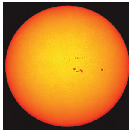
The sun
