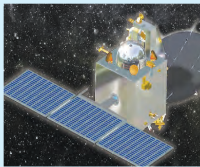
Mangalyaan
