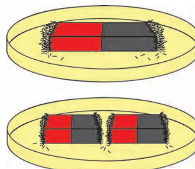
15.8 : Characteristics of magnetic poles
