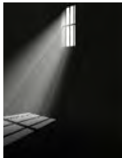
14.2 Light entering through a window
