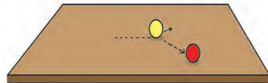
11.6 : Kinetic energy
