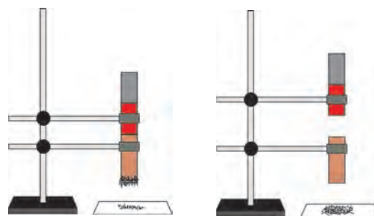
15.10 : Induced magnetism
