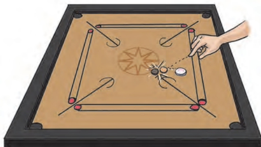
10.8 : Frictional force
