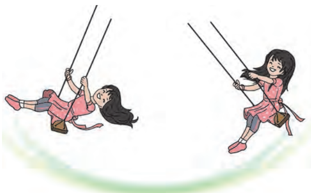
9.5 : Oscillatory motion
