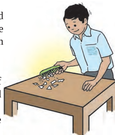
10.9 : Electrostatic force
