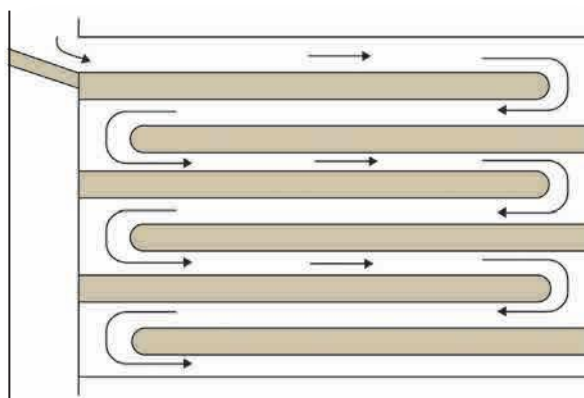
Fig. 2.3 Serpentine method
