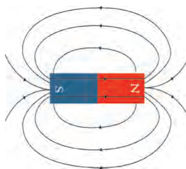
19.4 Magnetic field
