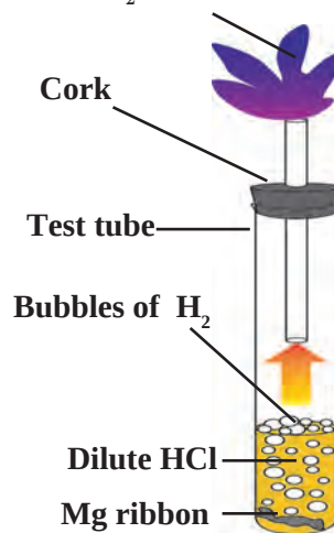
5.6 Reaction of a dilute solution of a strong acid with a metal
