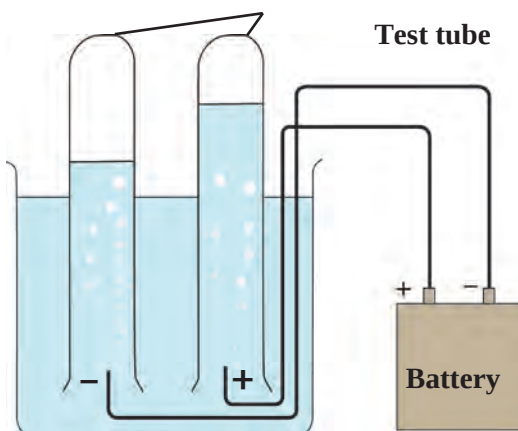
5.11 Electrolysis of water
