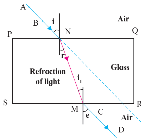
6.1 Refraction of light passing through a glass slab
