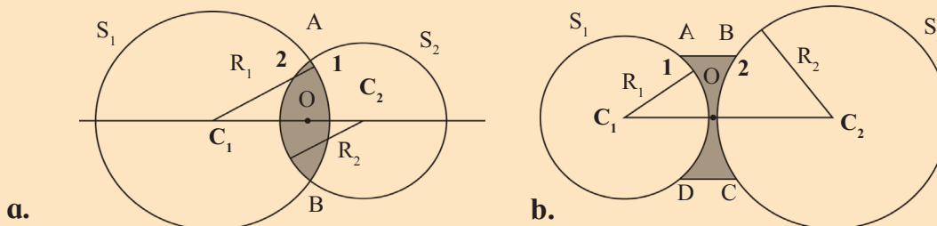
7.3 Cross-sections of convex and concave lenses.
