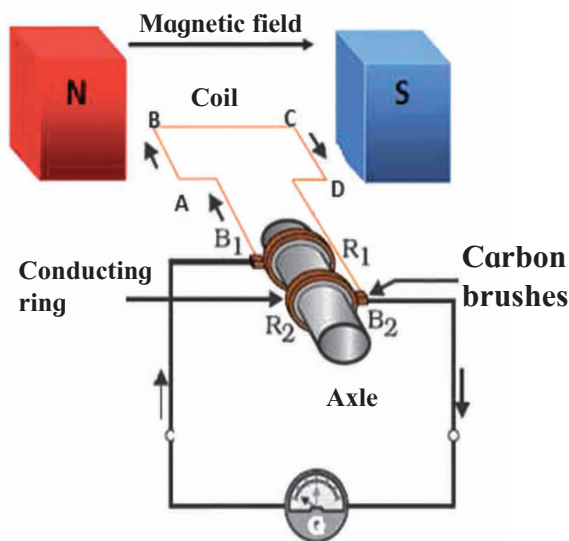
4.20 Electric generator
