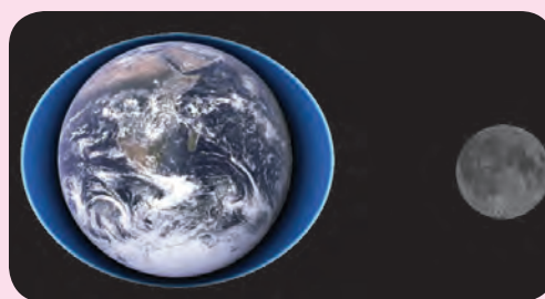
1.6 Low and high tides
