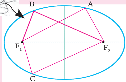
1.3 An ellipse
