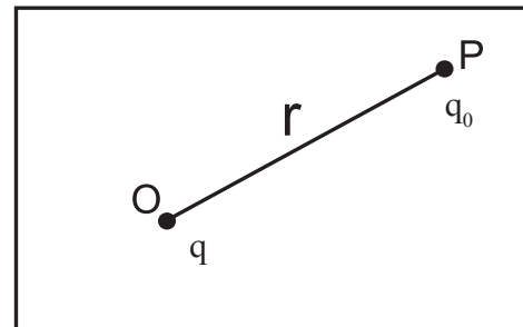
Fig. 10.7: Field in a material medium.
