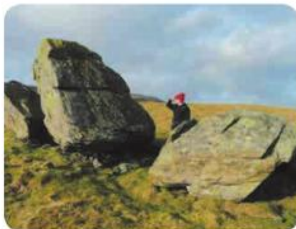
Fig. 3.36: Glacial erratics
