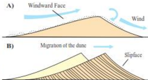
Fig. 3.23 : Migration of dunes
