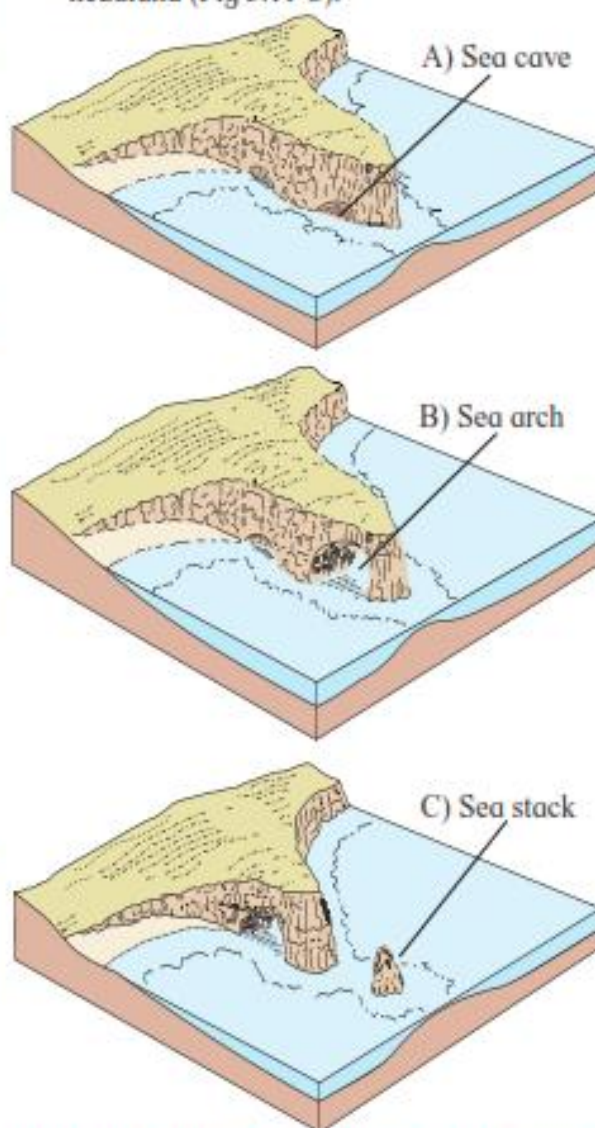
Fig. 3.11 : Sequence of development A) Sea cave, B) Sea arch, C) Sea stack
