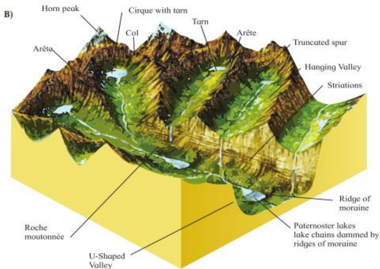
Fig. 3.33 : Glaciated terrain A) with glaciers, B) post glacier melting
