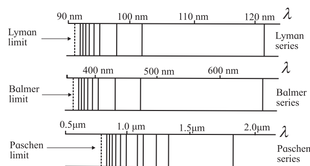
Fig.15.3: Lyman, Balmer and Paschen series in hydrogen spectrum.
