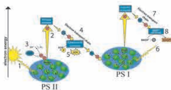
Fig. 12.8 Non-cyclic photophosphorylation
