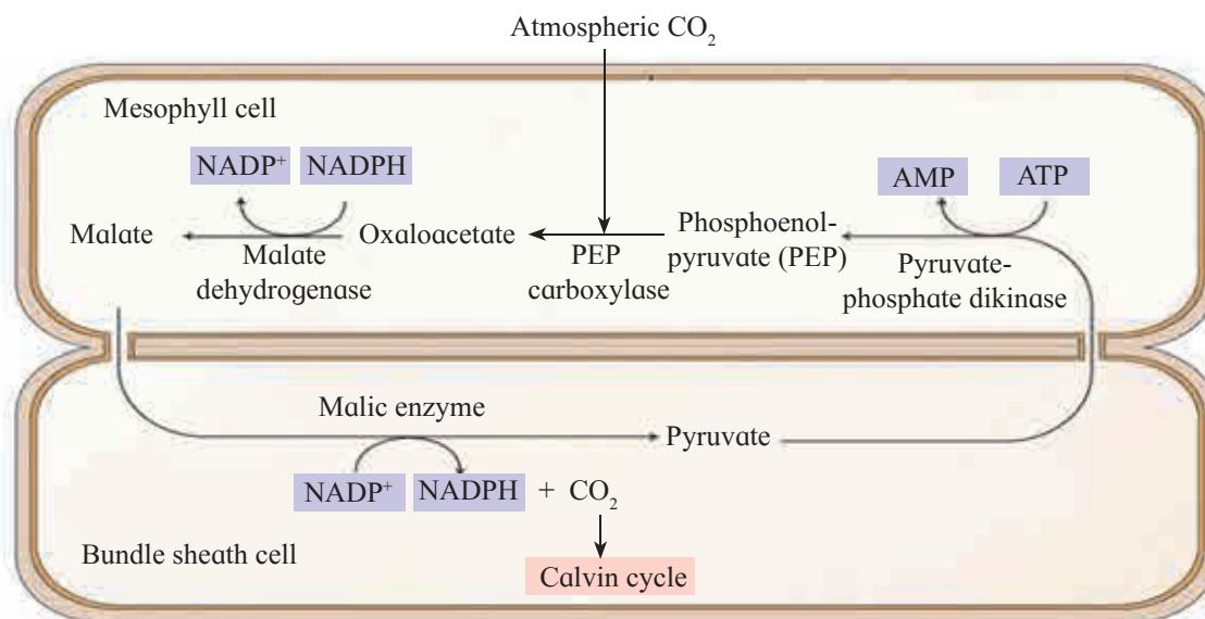
Fig. 12.13 C_4 Pathway
