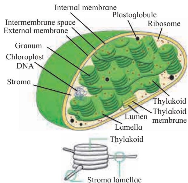
Fig. 12.1 Chloroplasts
