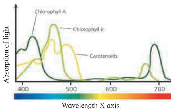
Graph 12.3 Absorption spectrum
