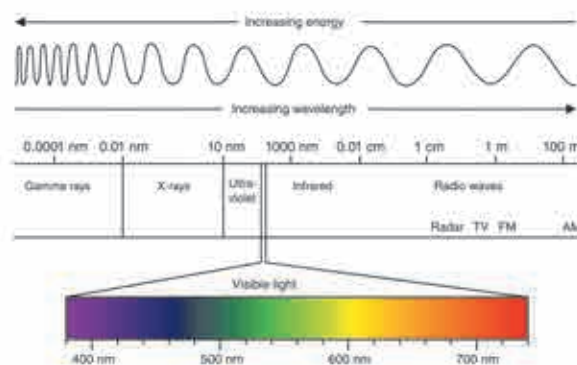
Fig. 12.2 Electromagnetic spectrum of light
