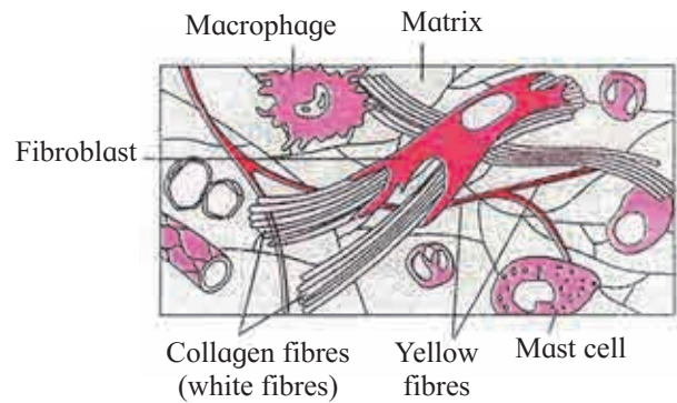
Fig. 10.9 Areolar tissue
