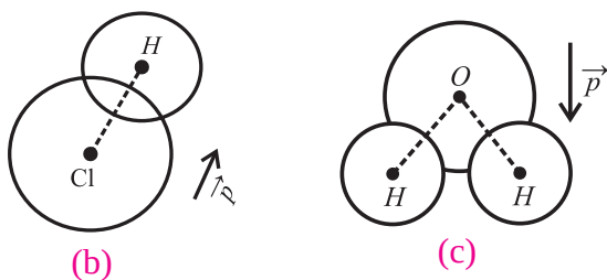
Fig. 8.18. Examples of Polar molecules (b) HCl (c) \text{H}_2\text{O} .
