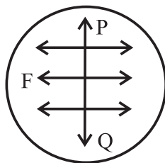
Fig. 2.16: Force of surface tension.
