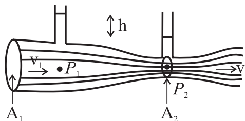
Fig. 2.36: Ventury tube.
