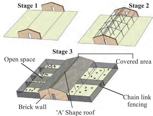
Fig. 4.2 : Ideal goat shed
