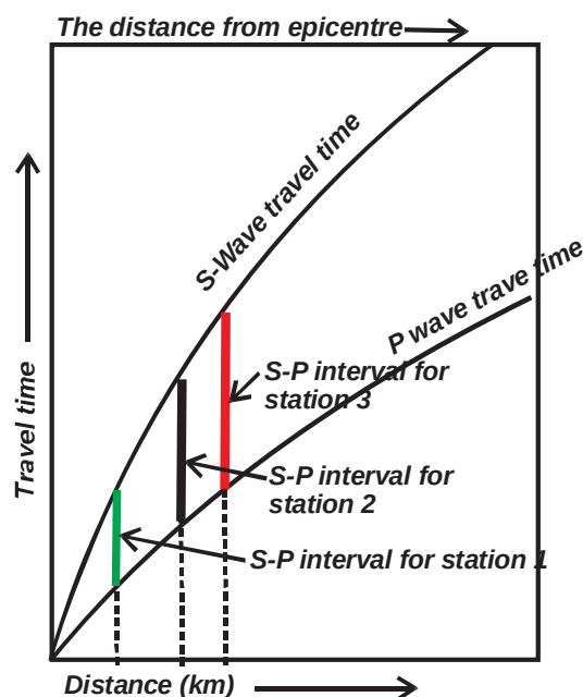
Fig. 7.9 : The concept of using standard travel-time graph to calculate the distance from station to epicentre using P-S time lag
