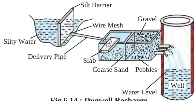
Fig.6.14 : Dugwell Recharge
