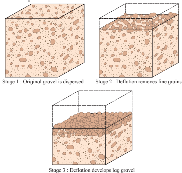
Fig. 3.16 : Formation of desert pavement / lag deposit
