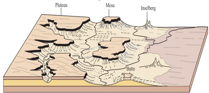
Fig. 3.20 : Mesa and butte
