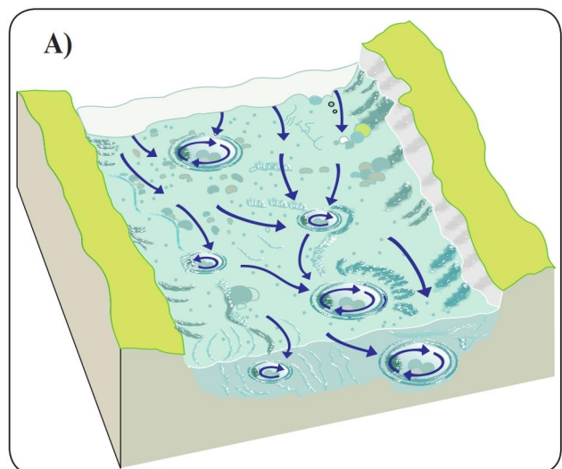
Fig. 3.1 : Zaskar valley, Jammu and Kashmir
