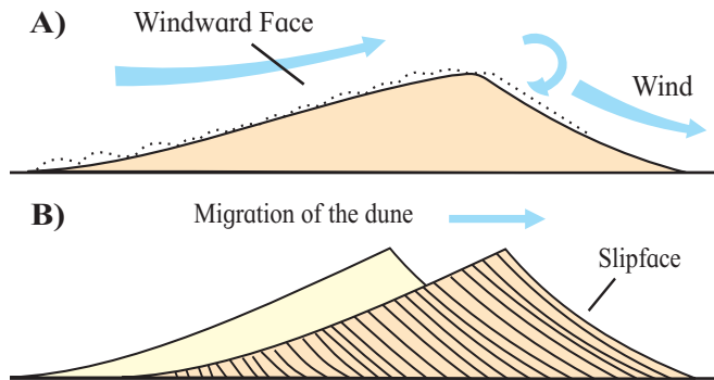
Fig. 3.23 : Migration of dunes
