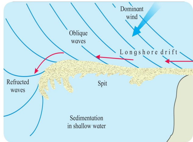
Fig. 3.13 : Formation of a Spit
