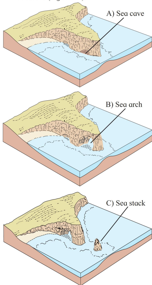
Fig. 3.11 : Sequence of development A) Sea cave, B) Sea arch, 3) Sea stack
