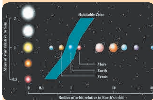
Depiction of Habitable Zone
