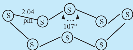
Structure of S 8 ring in rhombic sulfur
