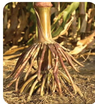
Fig. 9.10 Maize plant roots
