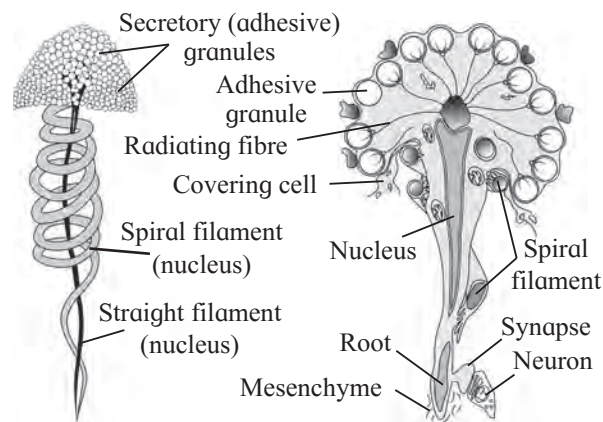
Colloblast
