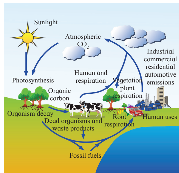
Fig. 14.10 : Carbon cycle
