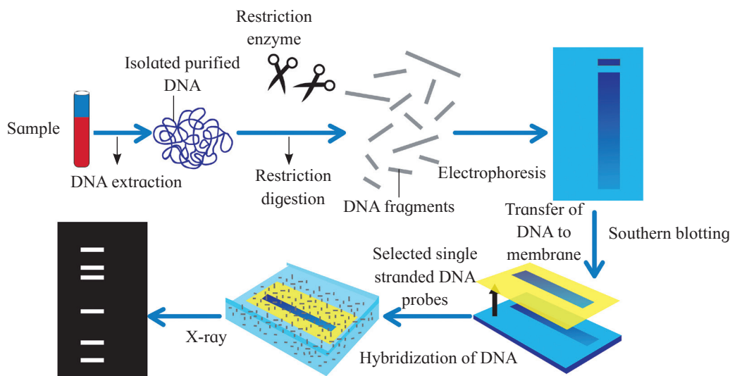
Fig. 4.18 : DNA Fingerprinting
