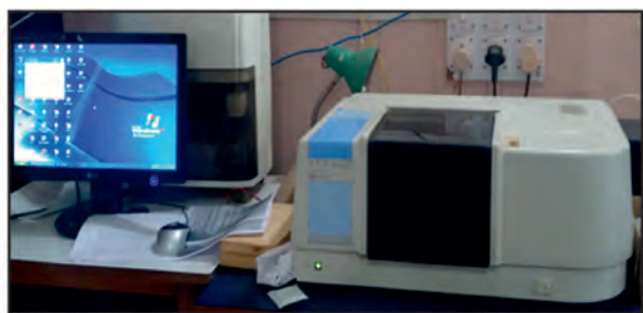
Fig. 16.12 FTIR spectroscopy
